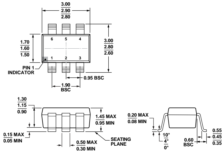
COMPLIANT TO JEDEC STANDARDS MO-178-AB Figure 70. 6-Lead Small Outline Transistor Package [SOT-23] (RJ-6)
