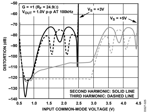
Figure 30. Harmonic Distortion vs. Input Common-Mode Voltage, \overline{DISABLE/SELECT} = Trisate\ or\ Open
