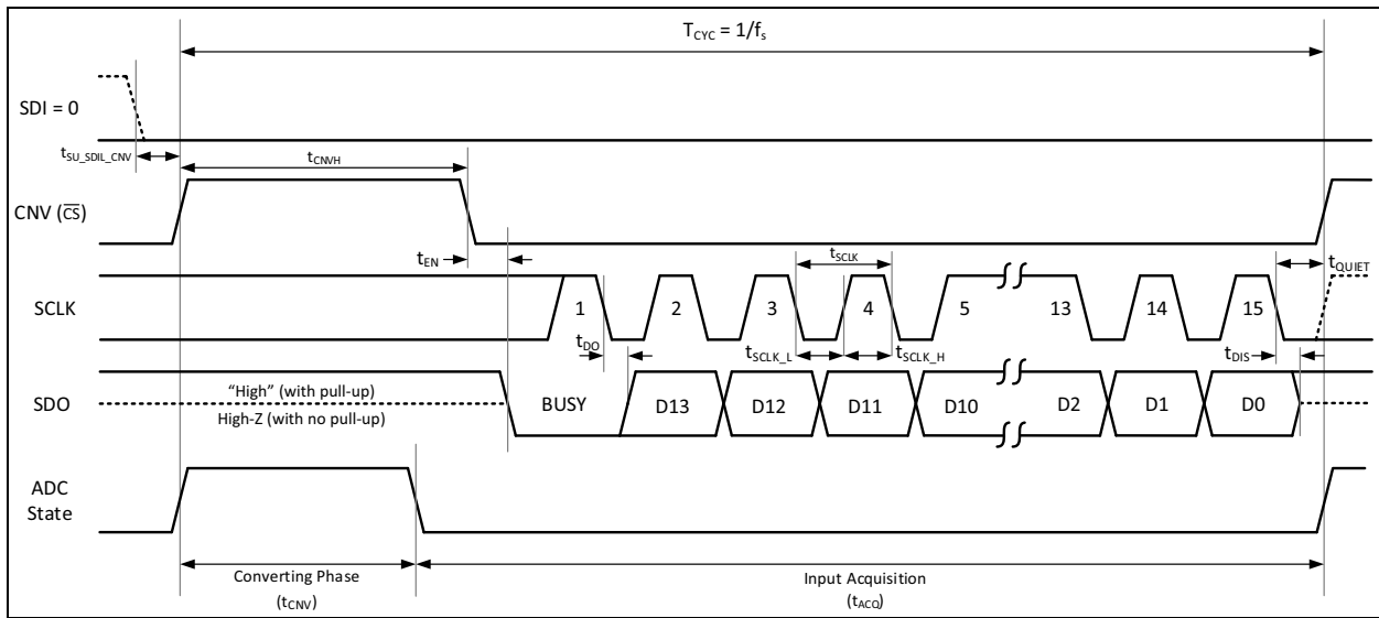
FIGURE 6-7: Timing Diagram for 3-Wire \overline{CNV} Mode with BUSY Status Indicator Output Bit, Late CNV.
