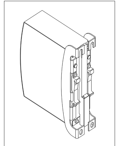
Fig. 22.1-3 Isometric view
