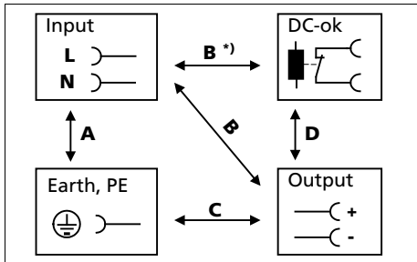
Fig. 18-1 Dielectric strength
