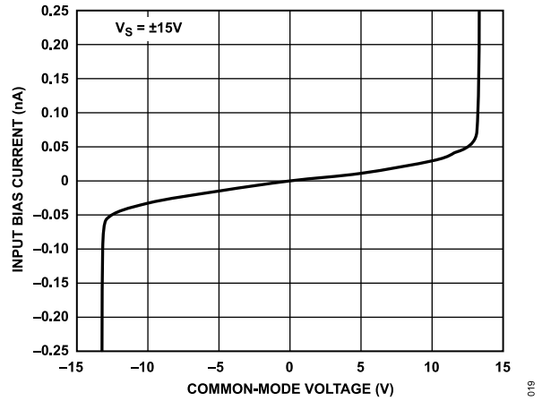
Figure 19. Input Bias Current vs. Common-Mode Voltage, V S = ±15 V
