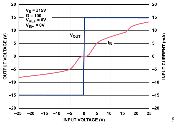
Figure 18. Input Overvoltage Performance; G = 100, V S = ±15 V
