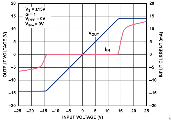
Figure 16. Input Overvoltage Performance; G = 1, V S = ±15 V
