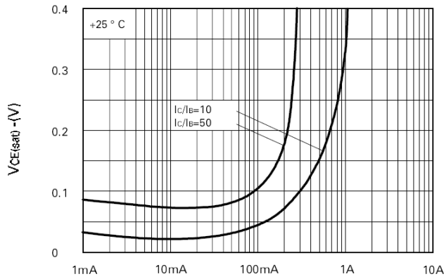
I C -Collector Current V CE(sat) v I C
