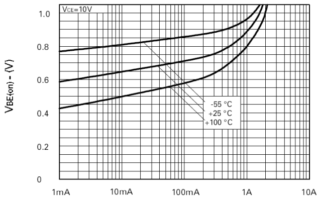
I C -Collector Current V BE(on) v I C
