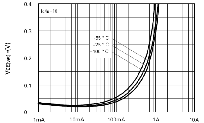
I C -Collector Current V CE(sat) v I C
