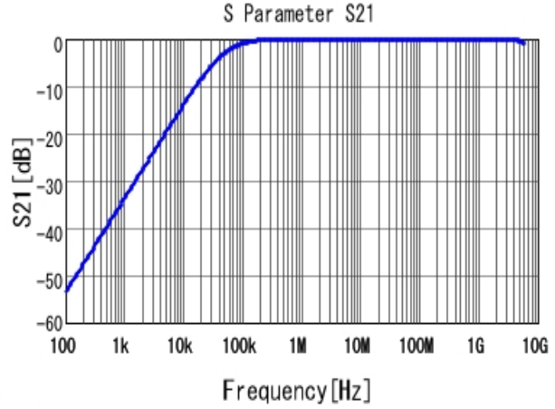
■ GCJ188R71H333KA12 S21 DCOV, 25degC
