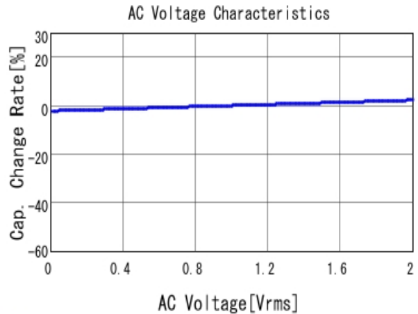
■ GCJ188R71H333KA12 C-AC Voltage capchange, DCOV, 25.0d
