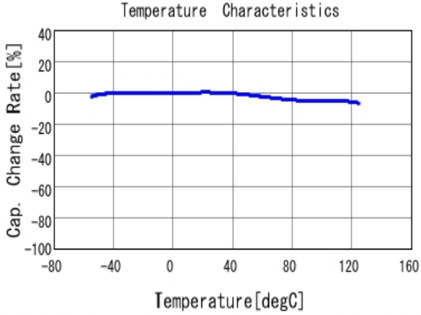
■ GCJ188R71H333KA12 C-Temp. capchange, DCO. 0V, AC1.0V rm
