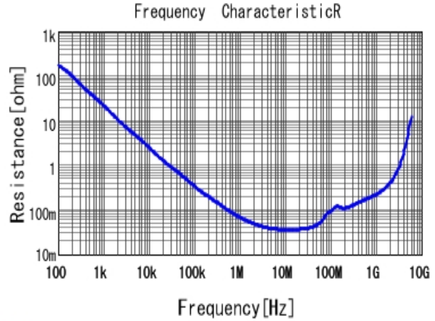
■ GCJ188R71H333KA12 R DCOV, 25degC
