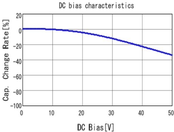
■ GCJ188R71H333KA12 C-DC bias capchange, 25.0degC, AC1.
