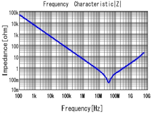
■ GCJ188R71H333KA12 |Z| DCOV, 25degC
