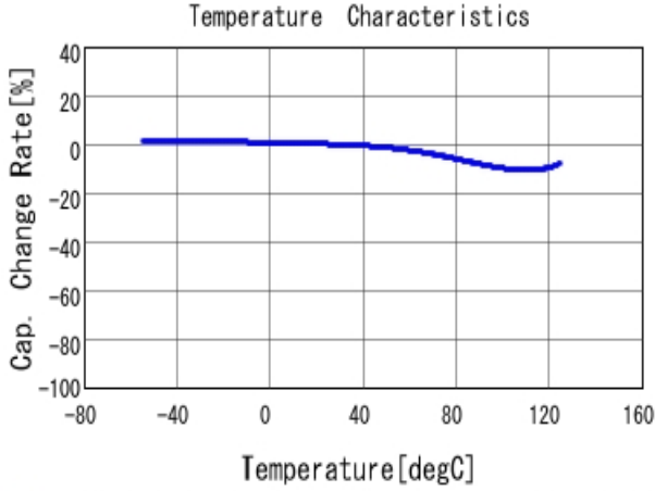
■ GCM188R72A682KA37 C-Temp. capchange, DCO. 0V, AC1.0Vrm
