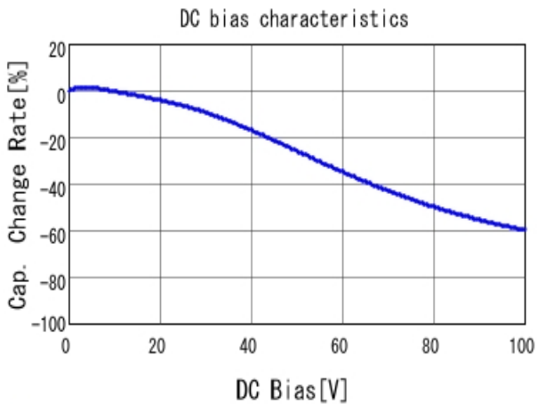
GCM188R72A682KA37 C-DC bias capchange, 25.0degC, AC1.
