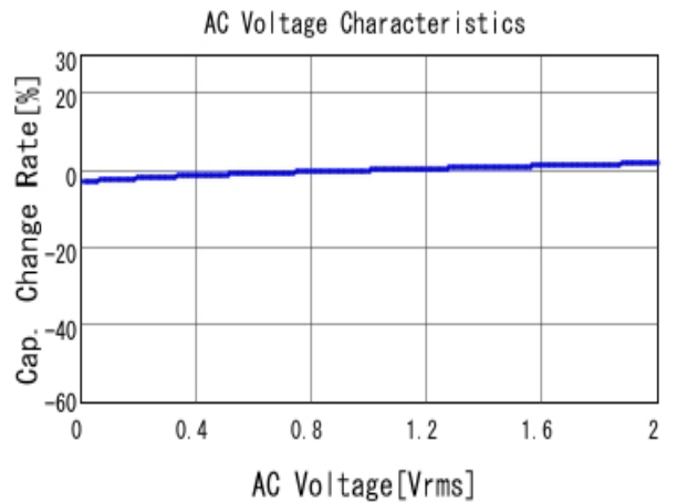
GCM188R72A682KA37 C-AC Voltage capchange, DCOV, 25.0d
