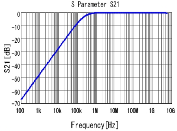
■ GCM188R72A682KA37 S21 DCOV, 25degC
