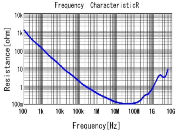
GCM188R72A682KA37 R DCOV, 25degC
