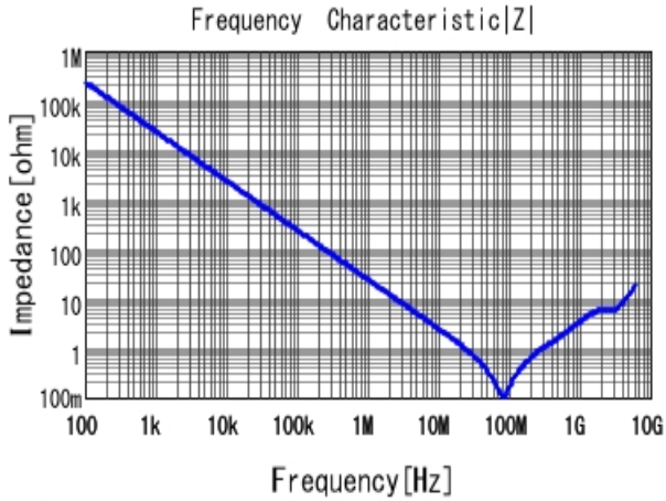
GCM188R72A682KA37 |Z| DCOV, 25degC
