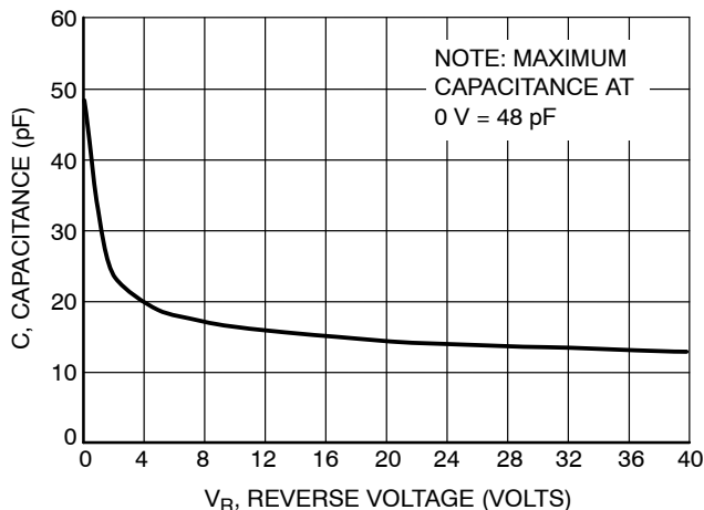
Figure 6. Maximum Capacitance
