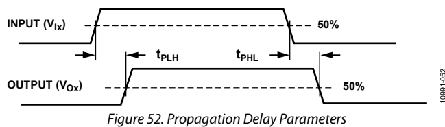
Figure 52. Propagation Delay Parameters
