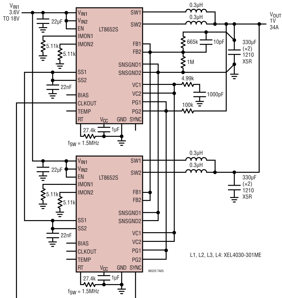
Four-Phase, 1V, 34A, 1.5MHz Step-Down Converter
