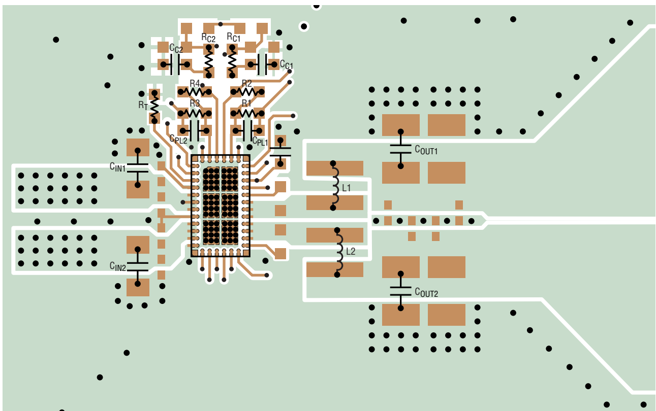
Figure 10. Recommended Layout
