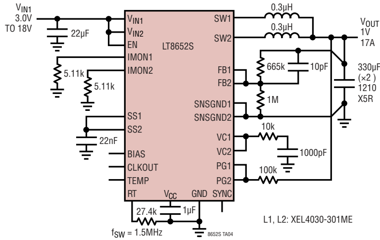
Two-Phase, 1V, 17A, 1.5MHz Step-Down Converter
