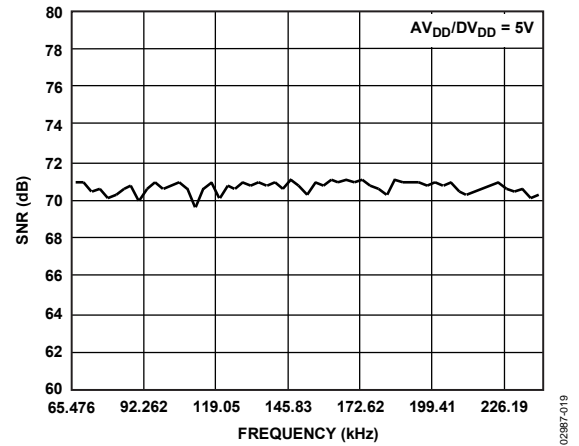
Figure 30. Typical Dynamic Performance vs. Sampling Frequency
