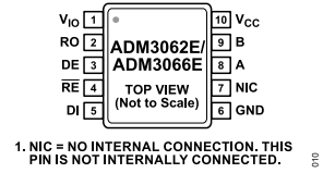
Figure 12. ADM3062E/ADM3066E 10-Lead MSOP Pin Configuration
