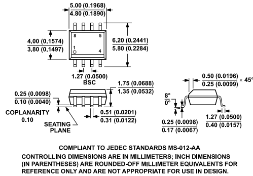
Figure 50. 8-Lead Standard Small Outline Package [SOIC_N] Narrow Body (R-8) Dimensions shown in millimeters and (inches)
