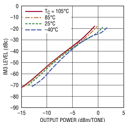
2-Tone IM3 Level vs Output Power Level
