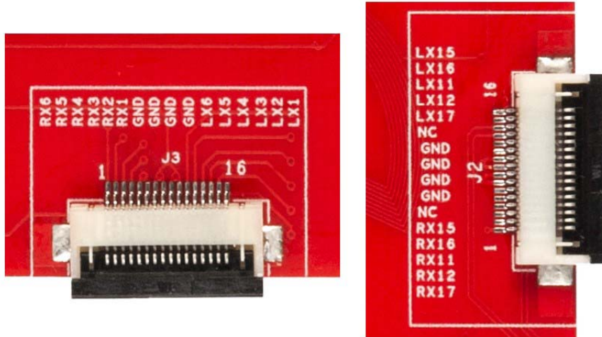
Figure A-4. On board FPC connectors
