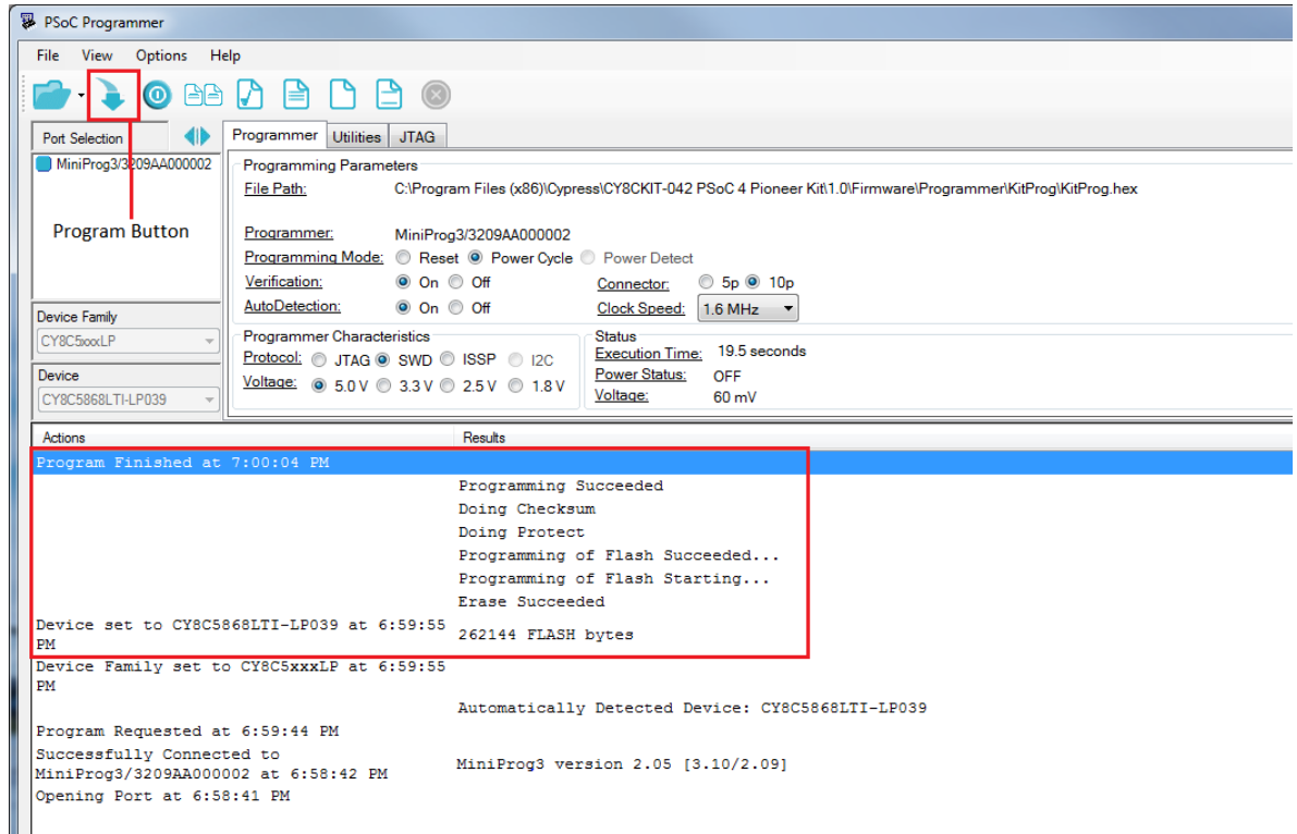
Figure 6-62. Program Finished
