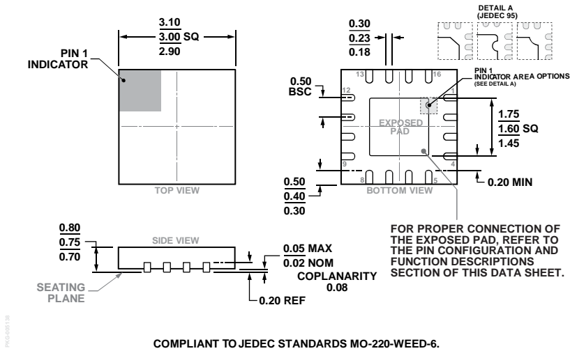
Figure 48. 16-Lead Lead Frame Chip Scale Package [LFCSP] 3 mm × 3 mm Body and 0.75 mm Package Height (CP-16-22) Dimensions shown in millimeters
