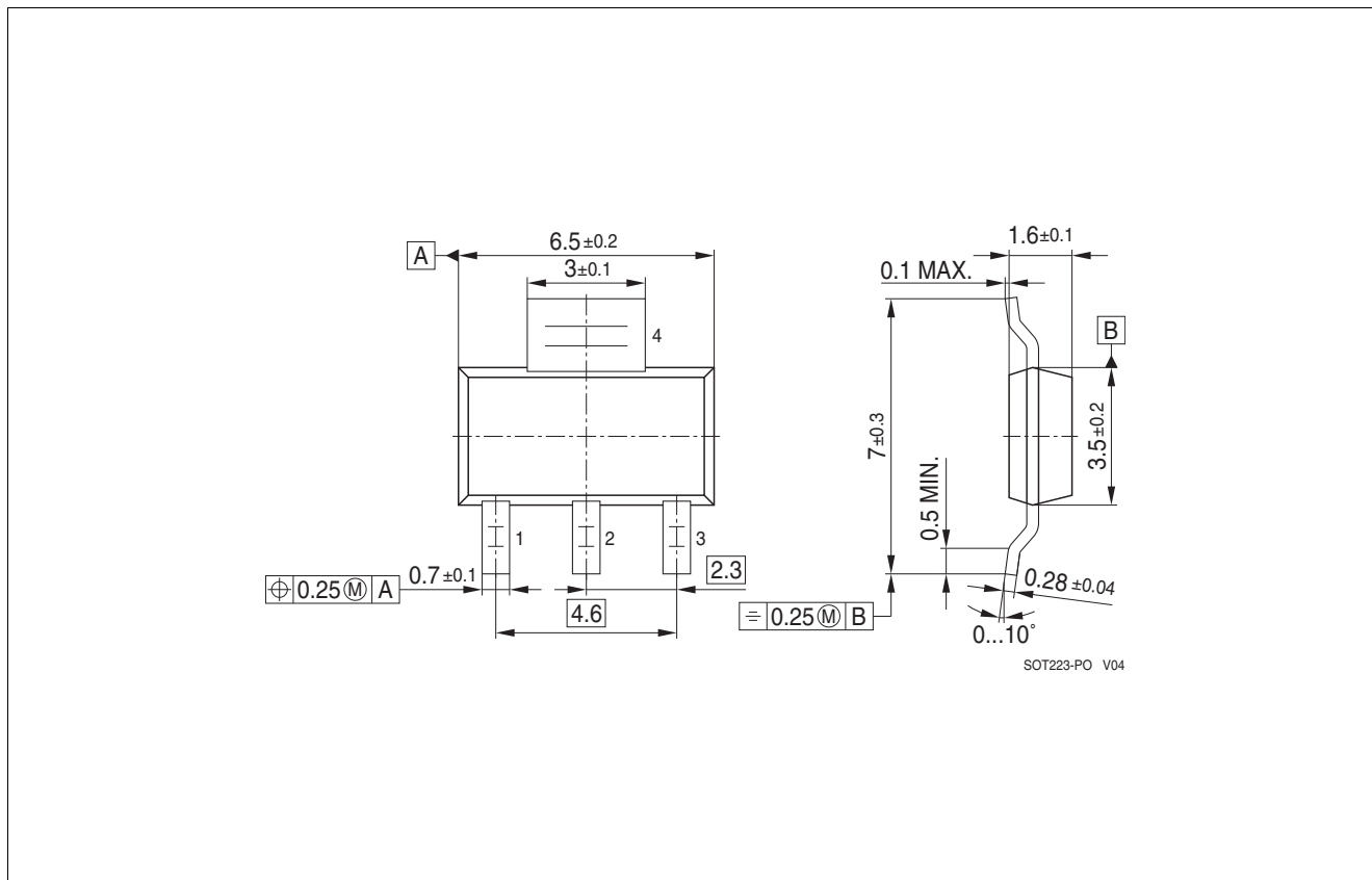
Figure 8 PG-SOT223-4
