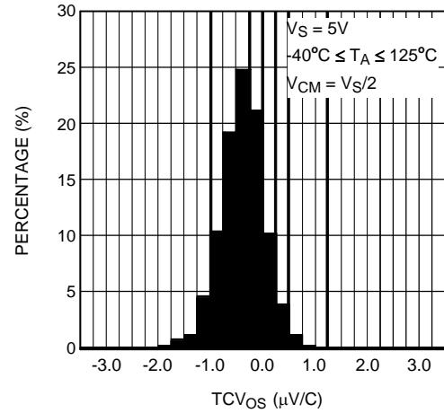
Figure 8. T_{cvos} Distribution
