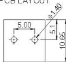
PCB LAYOUT
