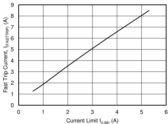
Figure 7-23. Fast Trip Threshold vs Current Limit
