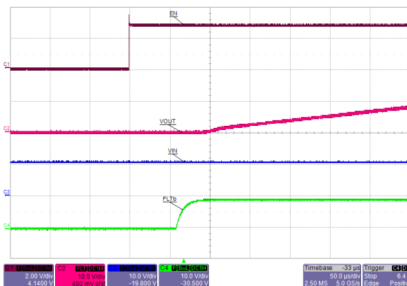
Figure 7-34. EN Turn ON Delay : EN \uparrow to Output Ramp \uparrow
