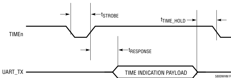
Figure 2. Timestamp Timing
