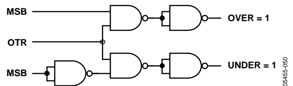
Figure 46. Overrange/Underrange Logic
