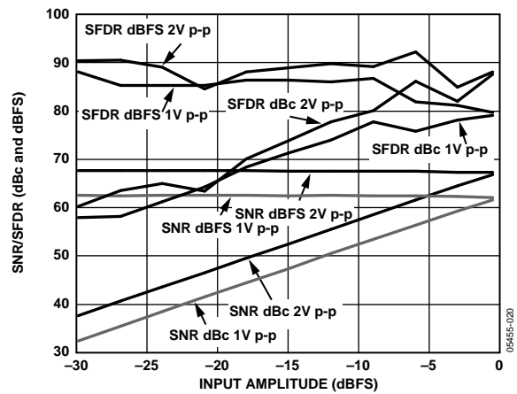
Figure 19. AD9237-20 SNR/SFDR vs. Input Amplitude with f_{IN} = 10 MHz
