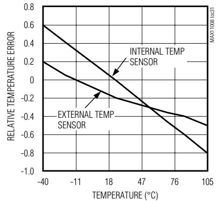
RELATIVE TEMPERATURE ERROR vs. TEMPERATURE
