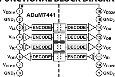
Figure 2. ADuM7441
