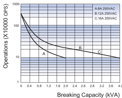
ENDURANCE CURVE
