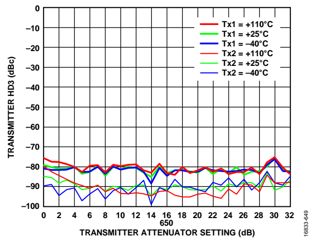
Figure 97. Transmitter HD3 vs. Transmitter Attenuator Setting, LO = 650 MHz, Digital Backoff = 15 dB
