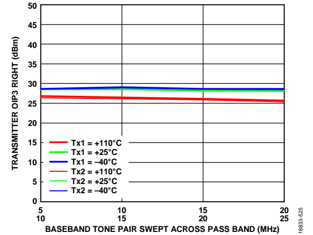
Figure 21. Transmitter OIP3 Right vs. Baseband Tone Pair Swept Across Pass Band, LO = 75 MHz, Total RMS Power = -12 dBFS, Transmitter Attenuation = 4 dB
