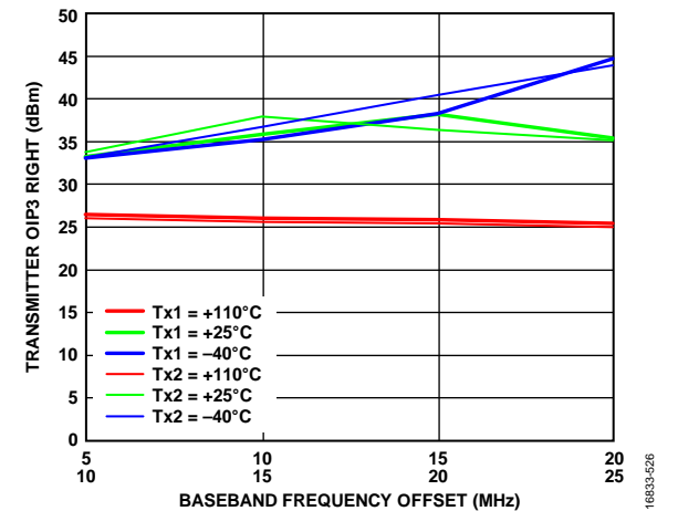
Figure 22. Transmitter OIP3 Right vs. Baseband Frequency Offset, LO = 300 MHz, Total RMS Power = -12 dBFS, Transmitter Attenuation = 4 dB
