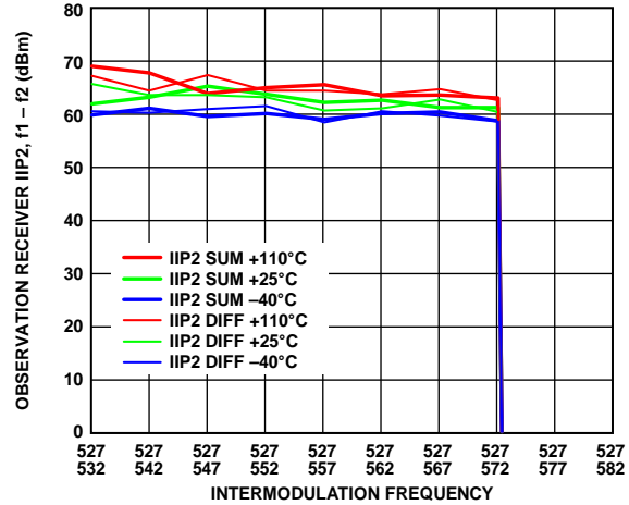
Figure 51. Observation Receiver IIP2, f_1 - f_2 vs. Intermodulation Frequency, LO = 525 MHz, Tone 1 = 527 MHz, Tone 2 = Swept, -25 dBm Each, Attenuation = 0 dB
