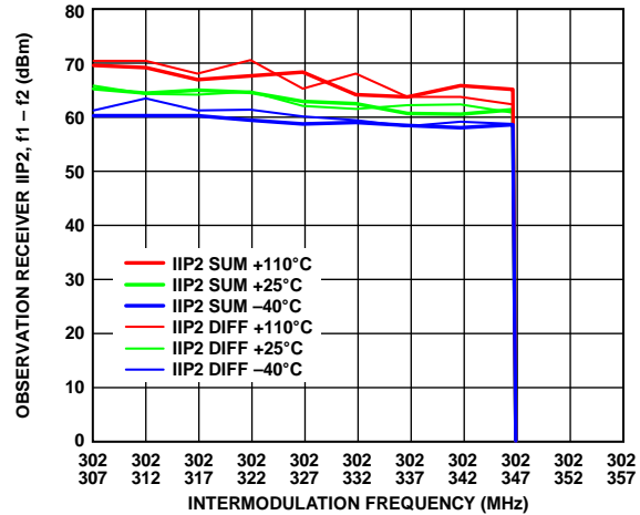
Figure 50. Observation Receiver IIP2, f_1 - f_2 vs. Intermodulation Frequency, LO = 300 MHz, Tone 1 = 302 MHz, Tone 2 = Swept, -25 dBm Each, Attenuation = 0 dB
