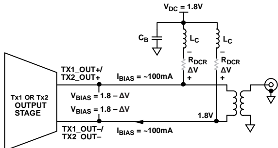
Figure 290. RF DC Bias Configurations Showing Parasitic Losses Due to Wire Wound Chokes
