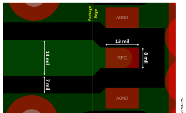
Figure 24. RF Transmission Lines
