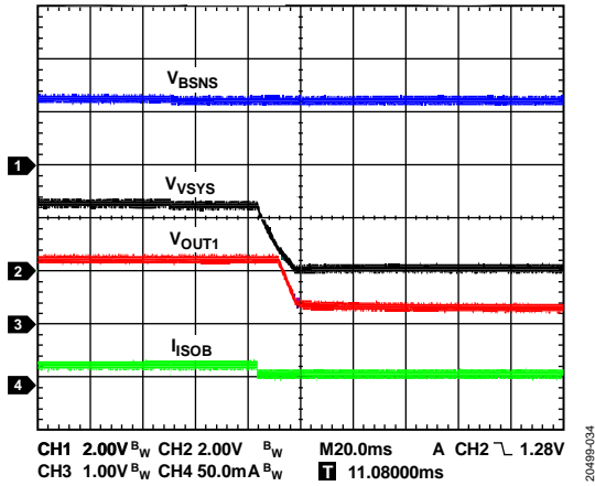
Figure 33. Battery Undervoltage Protection Waveform, V_{VBUS} = 0V , UV\_DISCH = 2.5V , DGT\_UV\_DISCH = 30\text{ ms}
