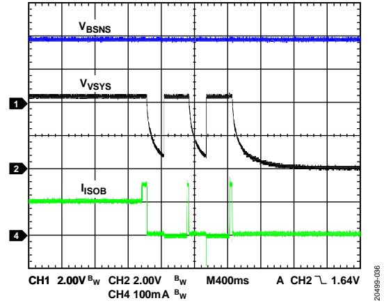
Figure 35. Battery Charge Overcurrent Waveform, V_{VBUS} = 5V , V_{ISOB} = 3.8V , OC\_CHG = 150\text{ mA} , DGT\_OC\_CHG = 10\text{ ms}
