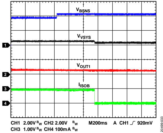
Figure 32. Battery Overvoltage Protection Waveform, V_{VBUS} = 5V , OV\_CHG = 4.3V , DGT\_OV\_CHG = 0.5\text{ sec}
