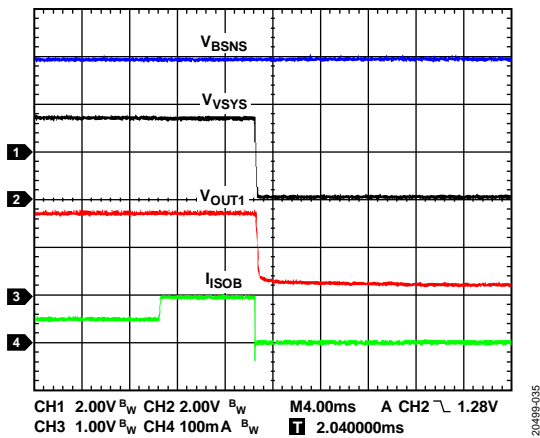
Figure 34. Battery Discharge Overcurrent Waveform, V_{VBUS} = 0V , V_{ISOB} = 3.8V , OC\_DISCH = 100\text{ mA} , DGT\_OC\_DISCH = 10\text{ ms}
