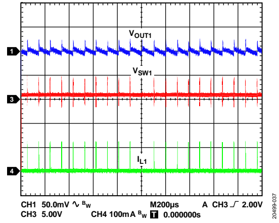
Figure 36. Buck Steady Hysteresis Waveform, Hysteresis Mode, V_{VIN2} = 3.8V , V_{OUT1} = 1.2V , Buck Output Current ( I_{OUT1} ) = 1 mA
