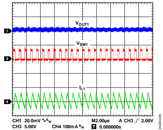
Figure 37. Buck Steady PWM Waveform, PWM Mode, V_{VIN1} = 3.8V , V_{OUT1} = 1.2V , I_{OUT1} = 1\text{ mA}
