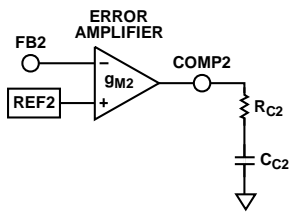
Figure 45. Compensation Component
