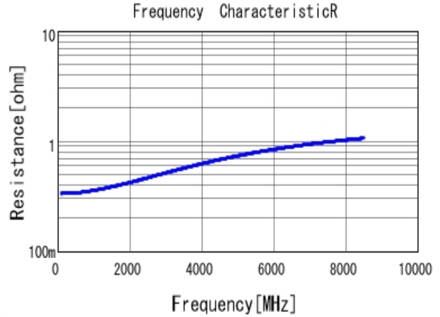
■ GRM0335C1H1R2CA01 R DC0V, 25degC
