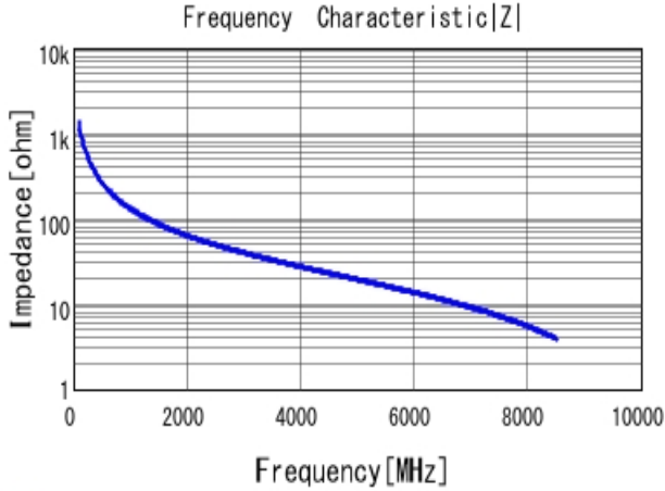
■ GRM0335C1H1R2CA01 |Z| DC0V, 25degC
