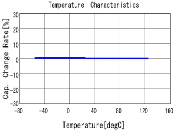
■ GRM0335C1H1R2CA01 C-Temp. capchange, DCOV, AC1Vrms
