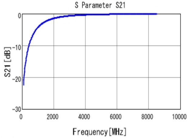
■ GRM0335C1H1R2CA01 S21 DCOV, 25degC
