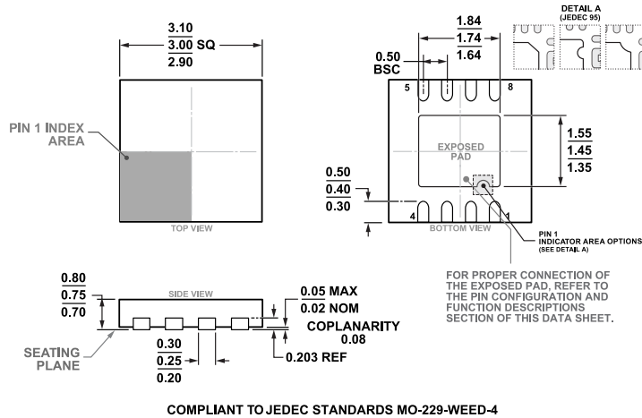
Figure 44. 8-Lead Frame Chip Scale Package [LFCSP] 3 mm x 3 mm Body and 0.75 mm Package Height (CP-8-13) Dimensions shown in millimeters
