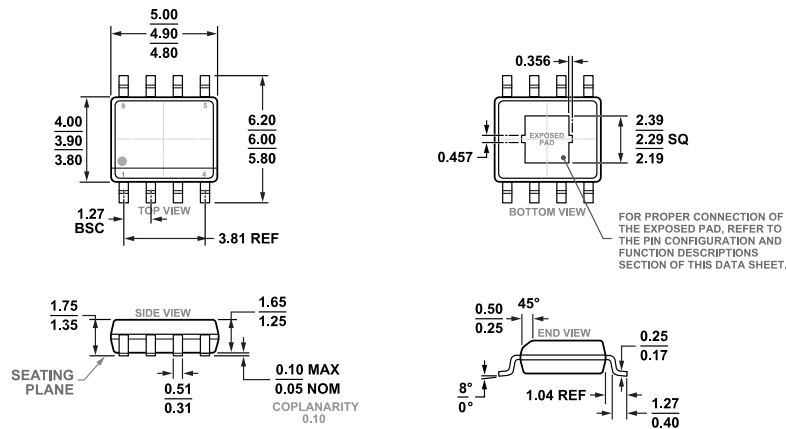
Figure 43. 8-Lead Standard Small Outline Package, with Exposed Pad [SOIC_N_EP] Narrow Body (RD-8-1) Dimensions shown in millimeters
