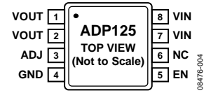
Figure 5. ADP125 Adjustable Output MSOP Pin Configuration
