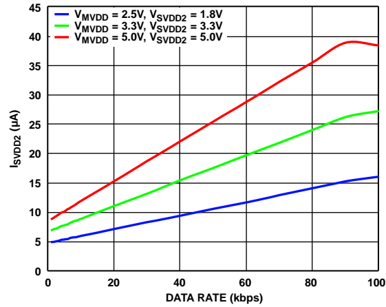
Figure 62. I_{SVDD2} Supply Current vs. Data Rate on All GPIO Channels at Various Supply Voltages, MSS High
