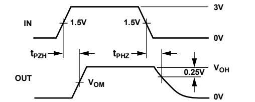
Figure 14. Driver Enable and Disable Times ( t_{PZH} , t_{PSH} , t_{PHZ} )
