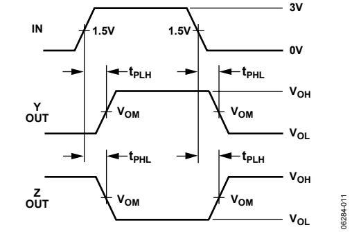
Figure 11. Driver Propagation Delays
