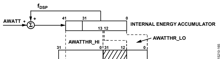
Figure 65. Internal Energy Register to AWATTHR_HI and AWATTHR_LO
