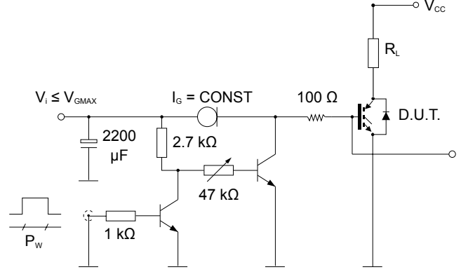
Figure 28. Gate charge test circuit
