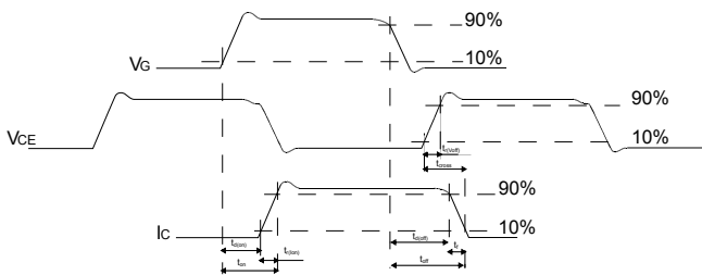
Figure 29. Switching waveform
