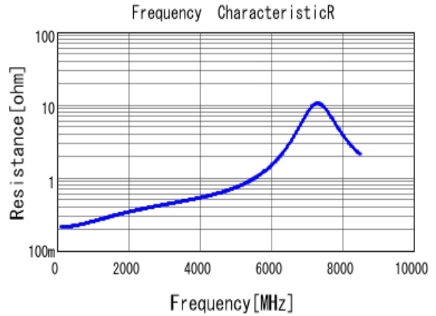
■ GRM1555C1H5R6WA01 R DCOV, 25degC
