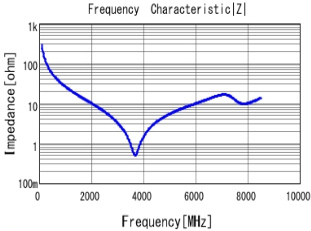
■ GRM1555C1H5R6WA01 |Z| DCOV, 25degC
