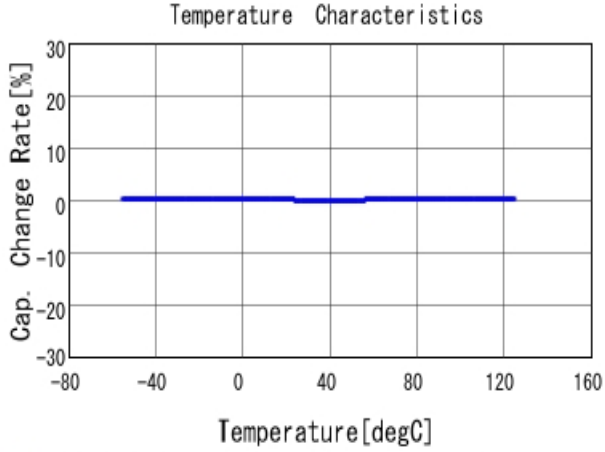
■ GRM1555C1H5R6WA01 C-Temp. capchange, DCOV, AC1Vrms
