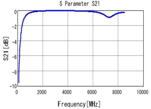
■ GRM1555C1H5R6WA01 S21 DCOV, 25degC
