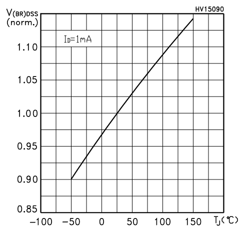
Figure 10. Normalized V_{(BR)DSS} vs temperature
