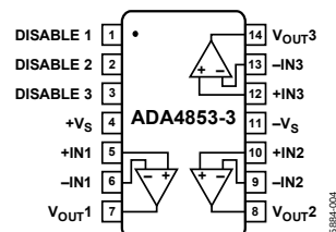
Figure 4. 14-Lead TSSOP
