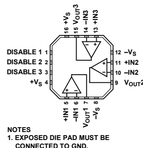
Figure 3. 16-Lead LFCSP_WQ
