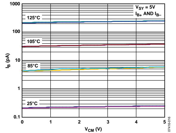
Figure 17. Input Bias Current vs. Common-Mode Voltage and Temperature
