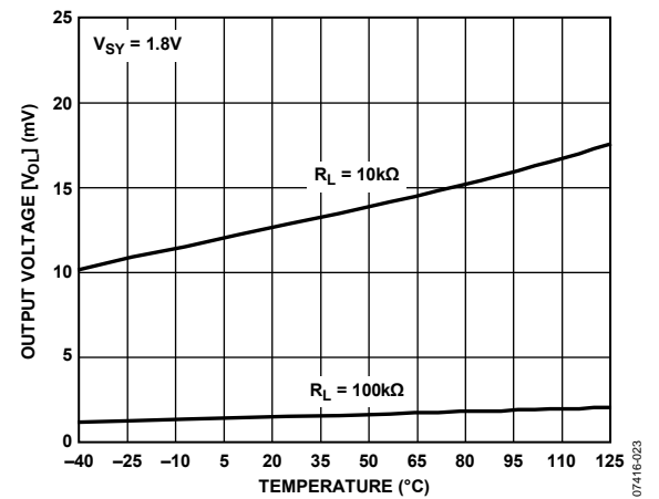
Figure 21. Output Voltage ( V_{OL} ) vs. Temperature
