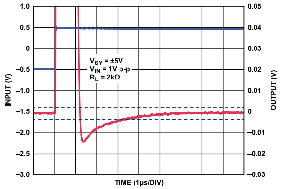
Figure 53. Positive 0.1% Settling Time, V_{SY} = \pm 5\text{ V}
