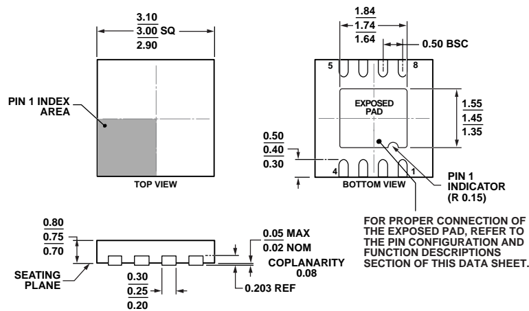
Figure 64. 8-Lead Lead Frame Chip Scale Package [LFCSP] 3 mm x 3 mm Body and 0.75 mm Package Height (CP-8-13)
