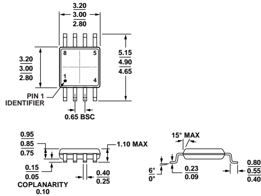
Figure 63. 8-Lead Mini Small Outline Package [MSOP] (RM-8)
