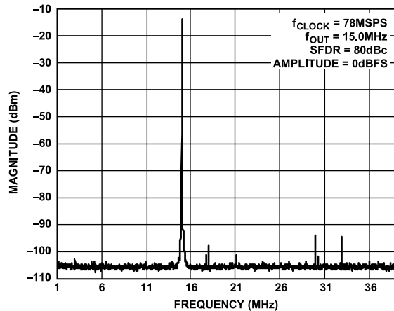
Figure 24. Single-Tone SFDR
