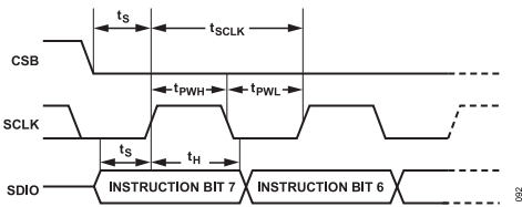
Figure 75. Timing Diagram for SPI Register Write
