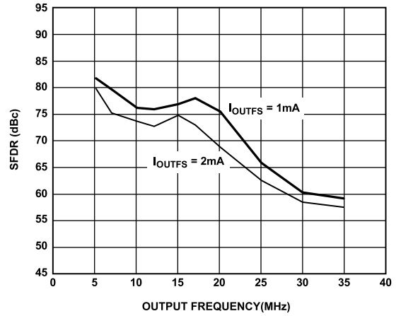
Figure 31. SFDR vs. f OUT and I OUTFS at 80 MSPS
