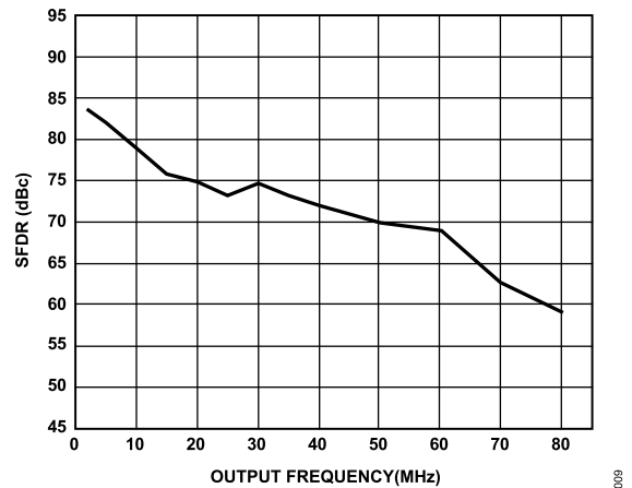
Figure 11. SFDR vs. f OUT at 175 MSPS
