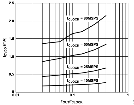
Figure 83. I_{DVDD} vs. f_{OUT}/f_{CLOCK} Ratio at DVDD = 1.8 V
