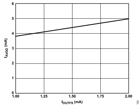
Figure 81. I AVDD vs. I OUTFS at AVDD = 1.8 V
