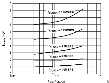
Figure 82. I DVDD vs. f OUT /f CLOCK Ratio at DVDD = 3.3 V
