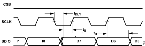
Figure 76. Timing Diagram for SPI Register Read
