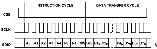
Figure 73. Serial Register Interface Timing, LSB First Write
