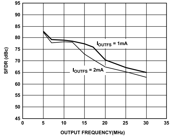
Figure 30. SFDR vs. f OUT and I OUTFS at 65 MSPS
