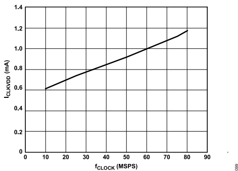
Figure 85. I_{CLKVDD} vs. f_{CLOCK} (Differential Clock Mode) at CLKVDD = 1.8 V
