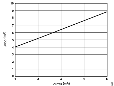
Figure 80. I AVDD vs. I OUTFS at AVDD = 3.3 V
