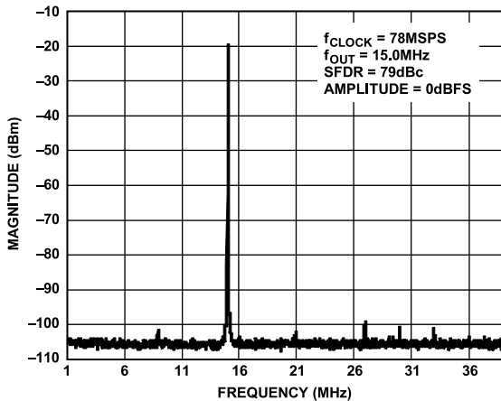
Figure 41. Single-Tone SFDR
