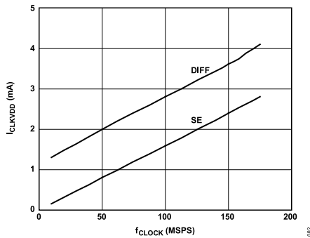
Figure 84. I_{CLKVDD} vs. f_{CLOCK} at CLKVDD = 3.3 V
