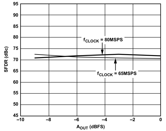
Figure 32. SFDR vs. A OUT at f OUT = f CLOCK /5
