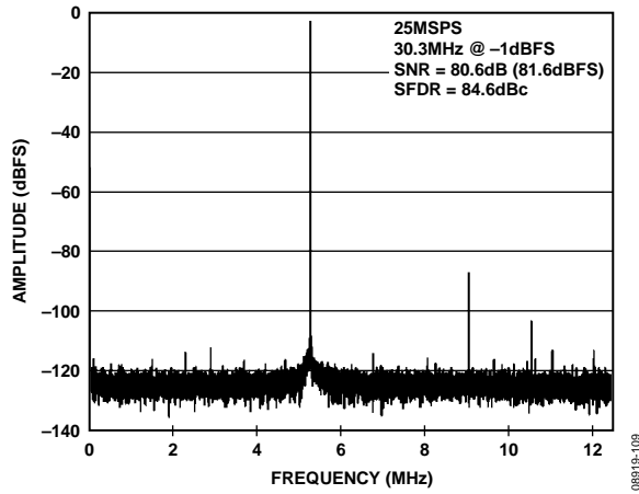
Figure 9. AD9650-25 Single-Tone FFT with f_{IN} = 30.3 MHz
