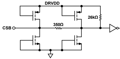
Figure 74. Equivalent CSB Input Circuit
