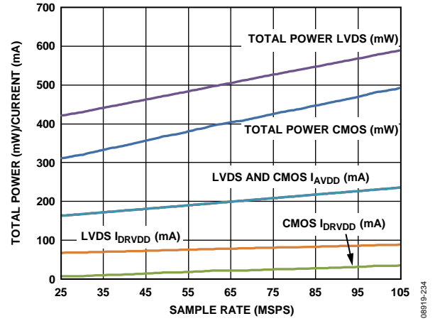
Figure 34. AD9650-65 Power and Current vs. Sample Rate
