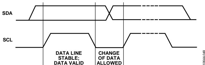
Figure 51. Valid Bit Transfer
