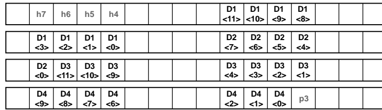
Figure 72. p3 Bit for 64-Bit Packet: 12-Bit Case
