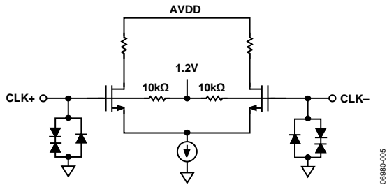
Figure 35. CLK± Inputs
