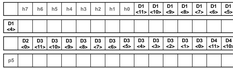
Figure 74. p5 Bit for 64-Bit Packet: 12-Bit Case
