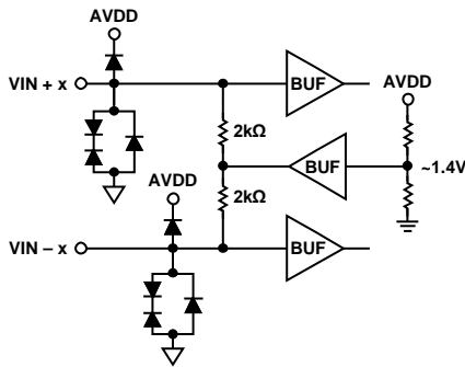
Figure 36. Analog Inputs
