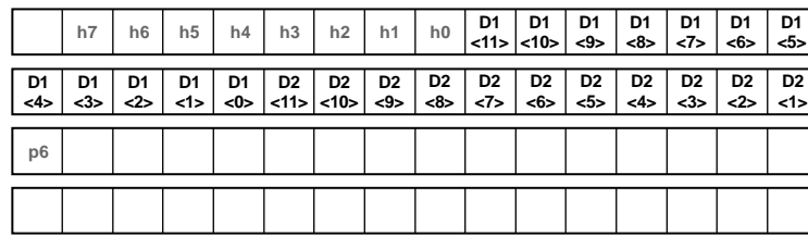
Figure 75. p6 Bit for 64-Bit Packet: 12-Bit Case
