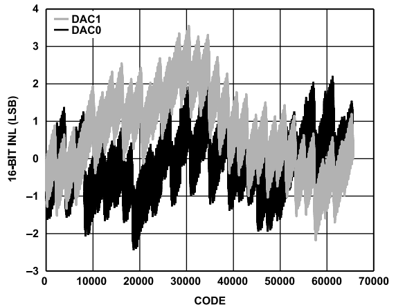
Figure 38. INL, I_{OUTFS} = 15.6 \text{ mA} , 16-Bit Resolution
