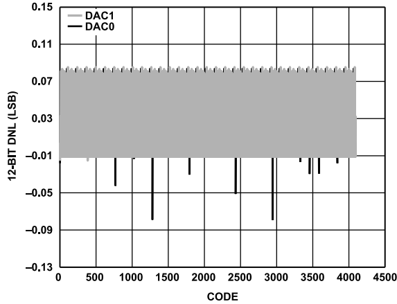
Figure 39. DNL, I_{OUTFS} = 20\text{ mA} , 12-Bit Resolution
