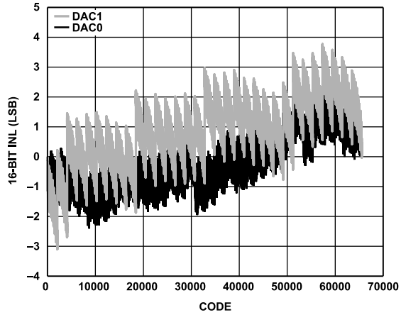
Figure 36. INL, I_{OUTFS} = 20 \text{ mA} , 16-Bit Resolution
