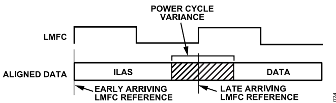
Figure 60. Link Delay > LMFC Period Example
