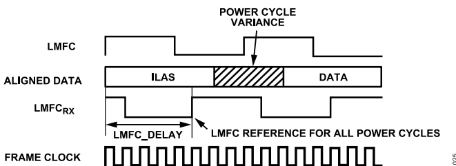
Figure 61. LMFC_DELAY_x to Compensate for Link Delay > LMFC
