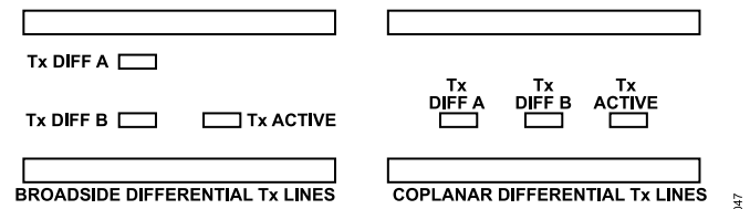
Figure 83. Broadside vs. Coplanar Differential Stripline Routing Techniques
