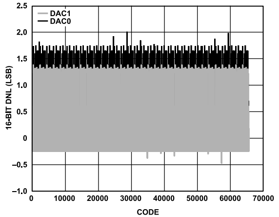
Figure 37. DNL, I_{OUTFS} = 15.6 \text{ mA} , 16-Bit Resolution
