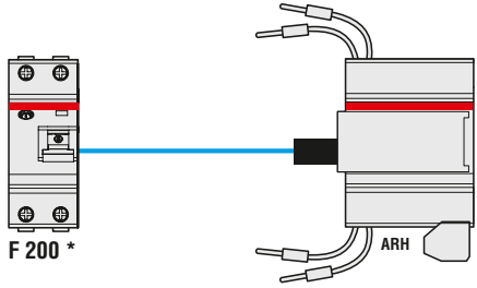
Combination of home automatic resetting unit with F200
