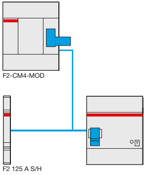
Combination of auxiliary elements with F204 125 A, F200 B high ratings
