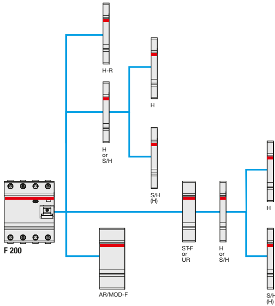
Combination of auxiliary elements with F200
