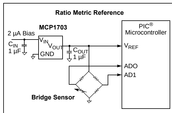
FIGURE 6-2: Using the MCP1703 as a Voltage Reference.
