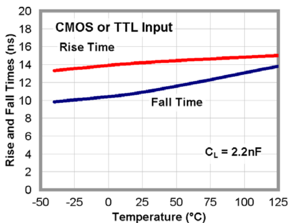
Figure 40. Rise and Fall Times vs. Temperature
